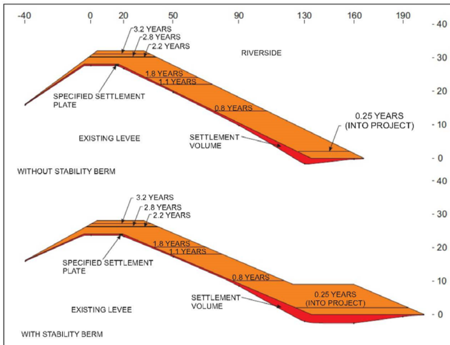
FIGURE 3: CALCULATED TOTAL SETTLEMENT DUE TO THE LEVEE ENLARGEMENT
