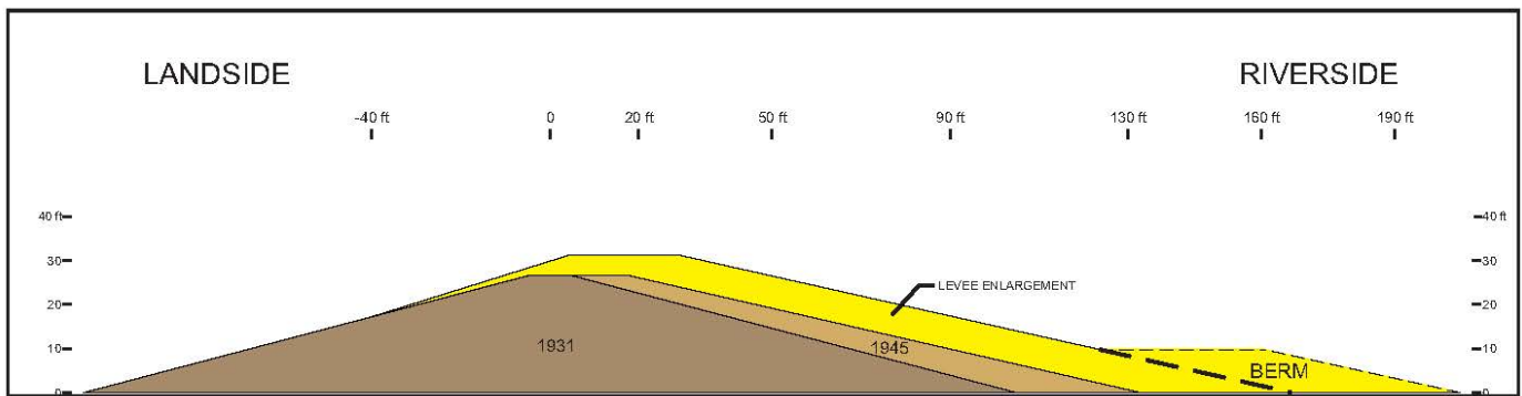
FIGURE 1: TYPICAL EXISTING AND PROPOSED ENLARGEMENT SECTIONS OF 7.75 MILE PROJECT LEVEE
