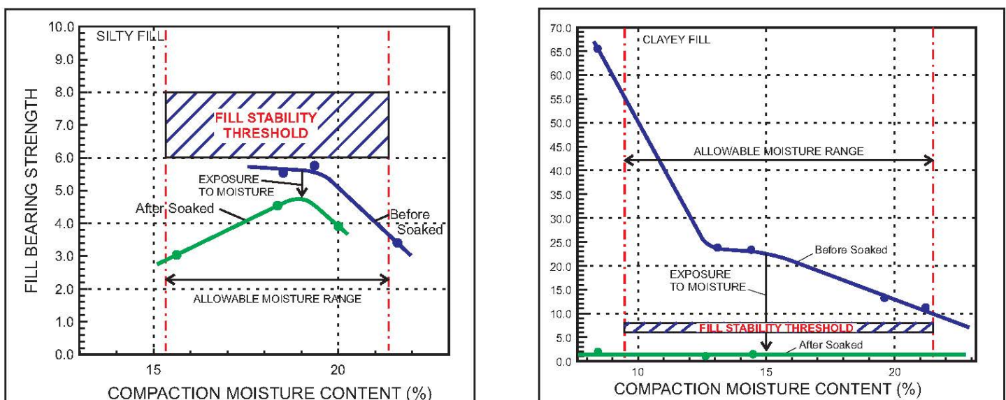
FIGURE 2: FILL STRENGTH WHEN COMPACTED UNDER CONDITIONS ALLOWED IN THE SPECIFICATIONS
