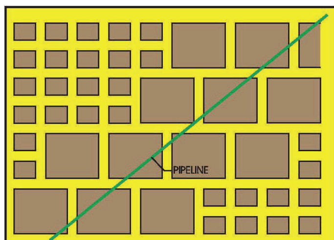
FIGURE 2 FINAL LAYOUT OF PILLAR SUPPORT USED BENEATH THE PIPELINE
