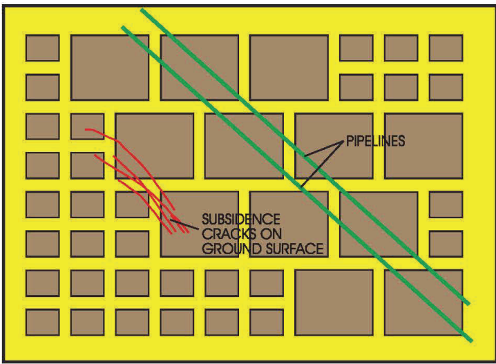
FIGURE 3 MINE SUBSIDENCE WITH SURFACE CRACKING TO LIMIT PILLAR SUPPORT FOR PIPELINES
