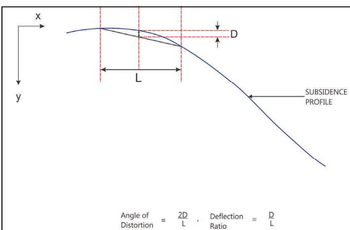
FIGURE 2 AVERAGE SLOPE AND ANGULAR DISTORTION (DEFLECTION RATIO) MEASUREMENTS ALONG A SUBSIDENCE PROFILE
