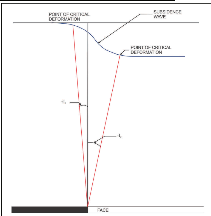
FIGURE 1 RELATIONSHIP OF LONGWALL FACE AND SUBSIDENCE WAVE
