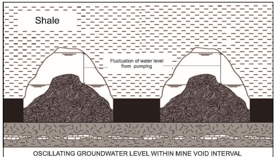
FIGURE 2 ROOF FAILURE ABOVE ROOM
