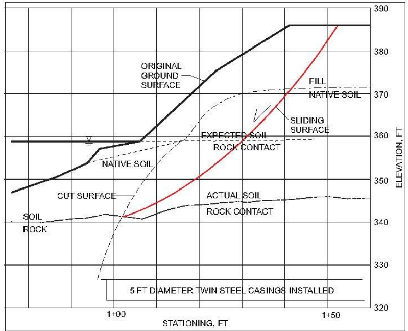
FIGURE 2 SOIL/ROCK PROFILE AT THE RIVERBANK
