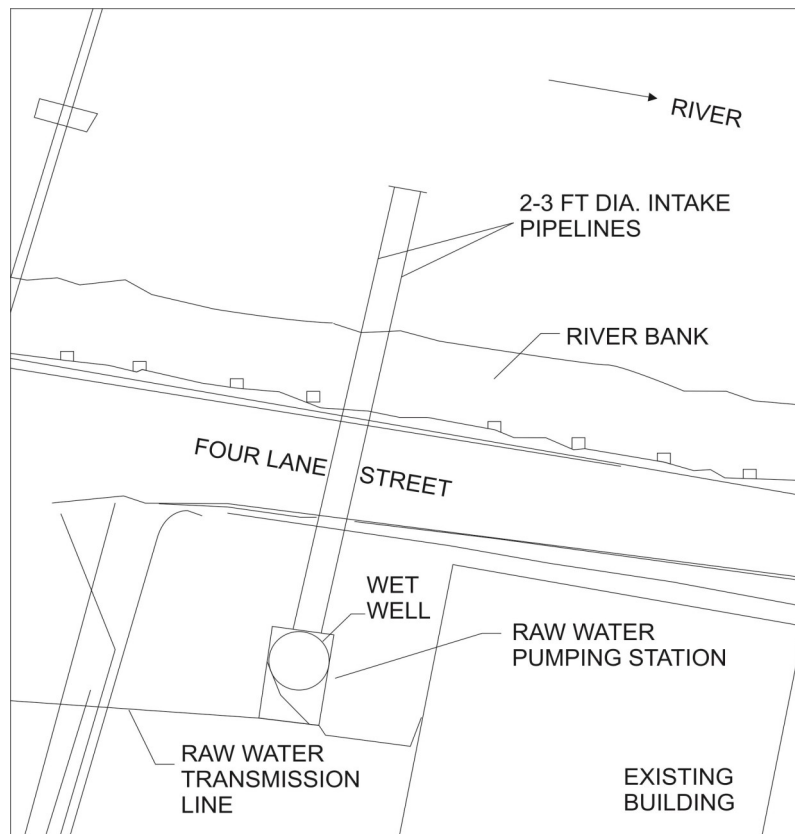
FIGURE 1 PLAN SHOWING THE LAYOUT OF THE WATER INTAKE FACILITY
