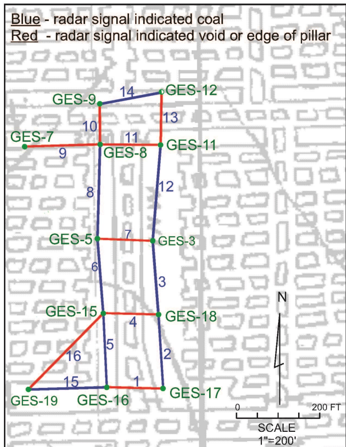
FIGURE 1 LOCATIONS OF DRILL HOLES AND CROSS-HOLE RADAR RAY PATHS SUPERIMPOSED OVER THE MINE MAP
