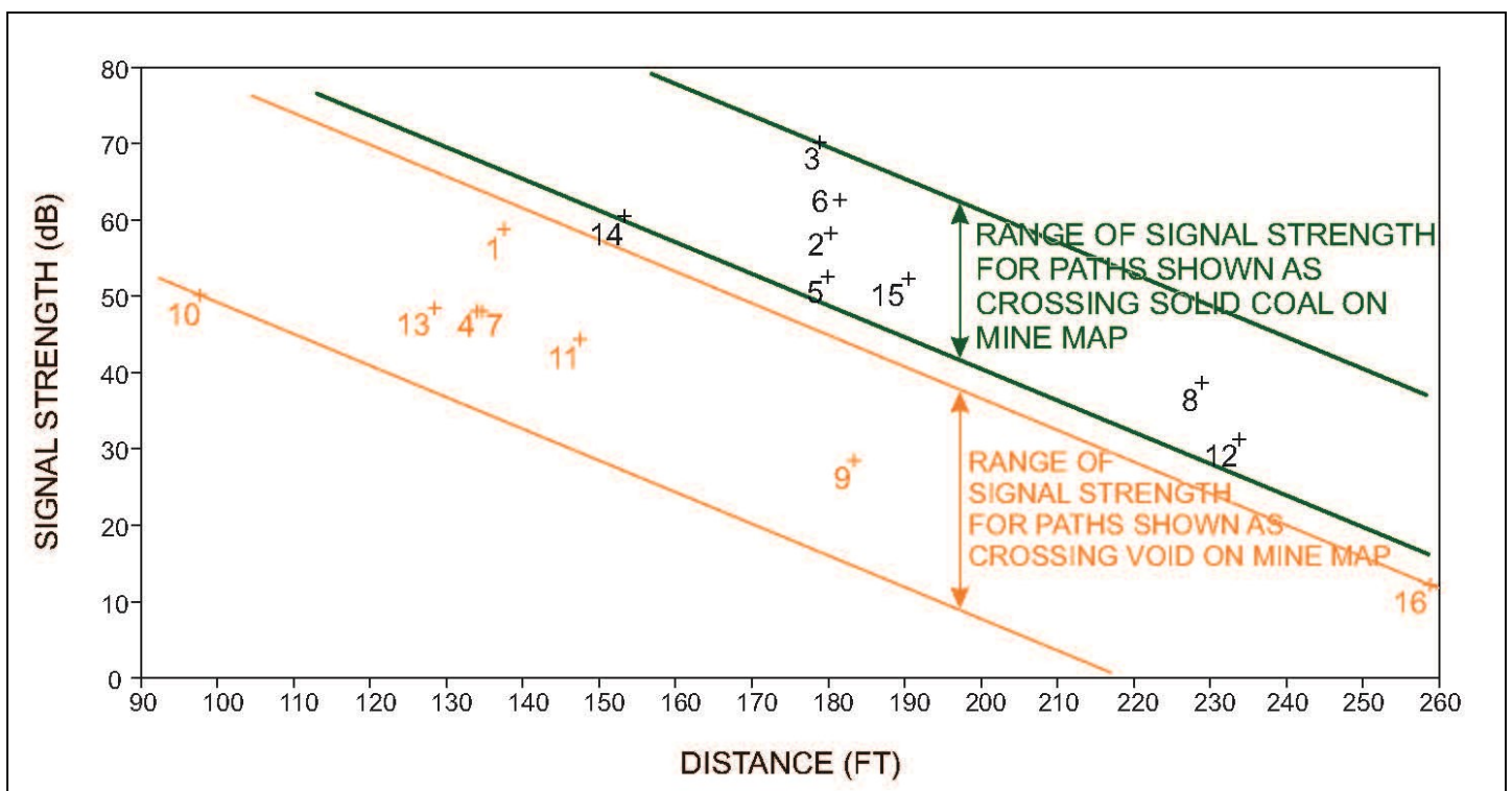
FIGURE 2 PLOT OF RADAR ATTENUATION RATES VERSUS RAY PATH DISTANCE
