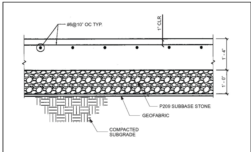
FIGURE 1: DESIGN CROSS-SECTION OF THE HANGAR SLAB
