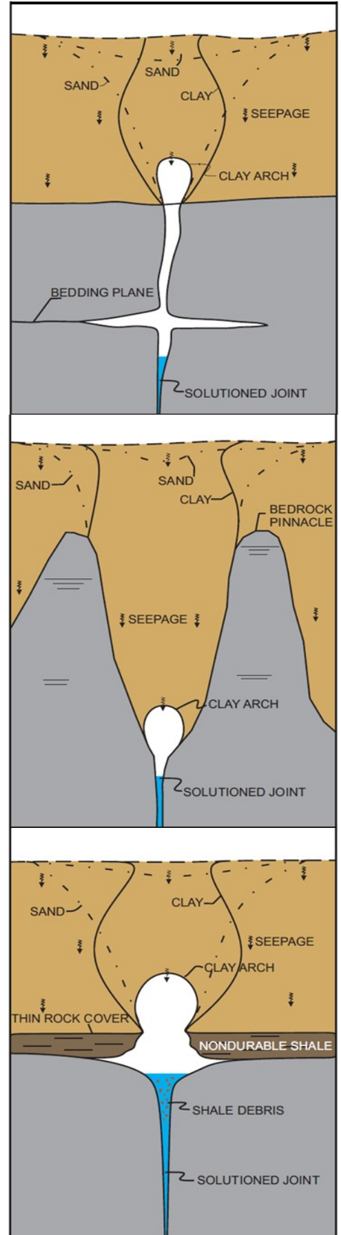
FIGURE 1 TYPICAL KARST SUBSIDENCE SCENARIOS
