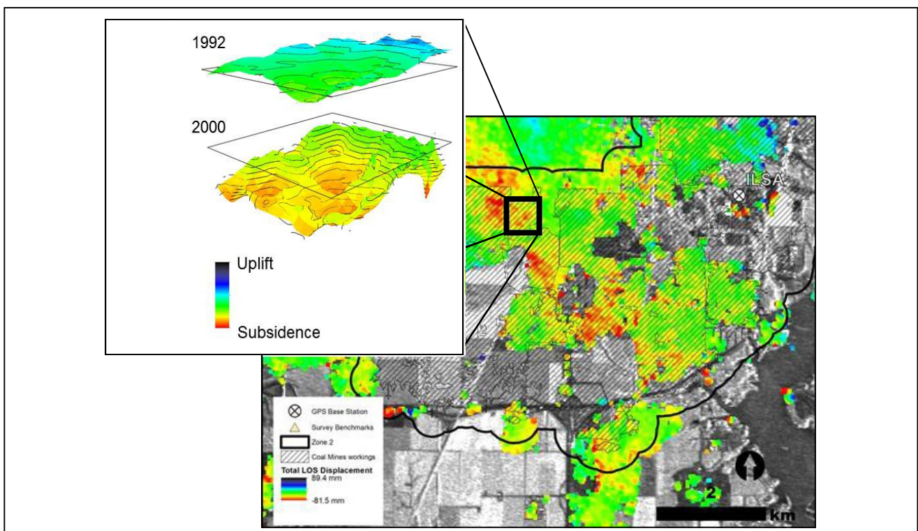
FIGURE 1 SUBSIDENCE HISTORY OF KNOWN SUBSIDENCE AREA IN SPRINGFIELD, IL
