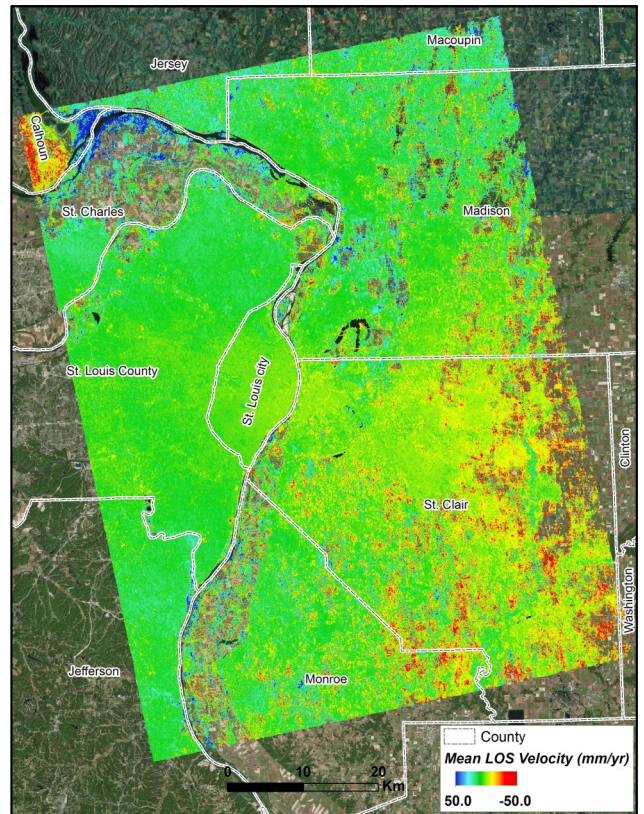
FIGURE 2 AVERAGE SUBSIDENCE 2006 TO 2010 OVER ST. LOUIS METRO AREA
