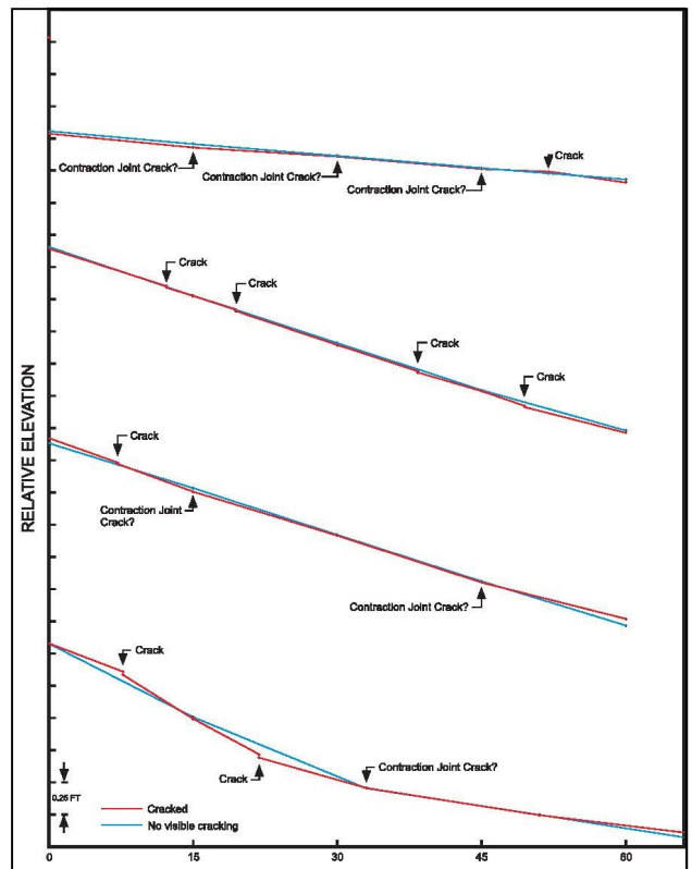
FIGURE 2 COMPARISON OF ELEVATION PROFILES ACROSS DAMAGED AND NEARBY UNDATED CONCRETE PAVEMENT SECTIONS
