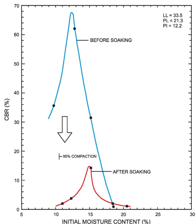
FIGURE 1 UNSOAKED AND SOAKED CBR VALUES VERSUS MOISTURE CONTENT AT STANDARD COMPACTION FOR SUBGRADE SOIL
